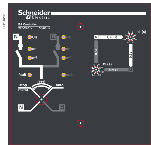
Front of the BA controller.
