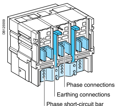
With short-circuit bar on the bottom connections.
